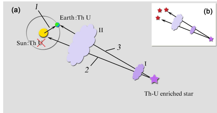
Figure 5. (a) The scheme illustrates a problem of the Th-U nucleosynthesis from the Th-U enriched star, nearest to the Earth. The nearest single neutron star is allocated at the distance of 167 pc from our solar system. Clouds I and II demonstrated reducing concentrations at the propagation in space; (b) property of invariance of isotopes for a group of neighborhood stars is shown on a plate.
