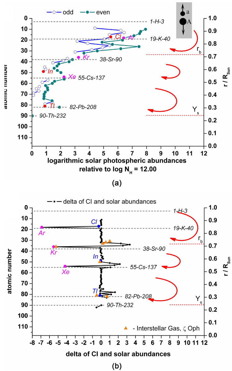
Figure 6. (a) The logarithmic solar abundances of elements in the solar photosphere are shown. In grey plate the theory of buoyancy schematically is shown: the light elements flow up and heavy elements sink down. (b) The delta of CI carbonaceous chondrites logarithmic abundance [15] and solar photosphere abundance [11] [12] [13] was presented. The indirect photospheric estimates have been used for the noble gases: Ar, Kr, Xe (magenta color). Abundances chlorine Cl, indium In, thallium Tl, obtained from sunspot spectrums, were presented as blue points. All values were calibrated to \log N_H = 12 . The red arrows demonstrated convection processes determined by helioseismological methods ( r_b , Y_s ). The delta between interstellar gas abundances ( \zeta -Oph) and CI meteorites was presented by orange triangles [76].
