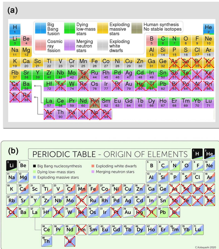
Figure 1. Two standard periodic tables, showing the origins of each chemical element. (a) periodic tables according to B 2 FH model (adapted from Wikipedia); (b) K 2 L model (Artwork: Sahn Keily). The red crosswise marks the elements which could not be recorded in the solar photosphere spectrum.
