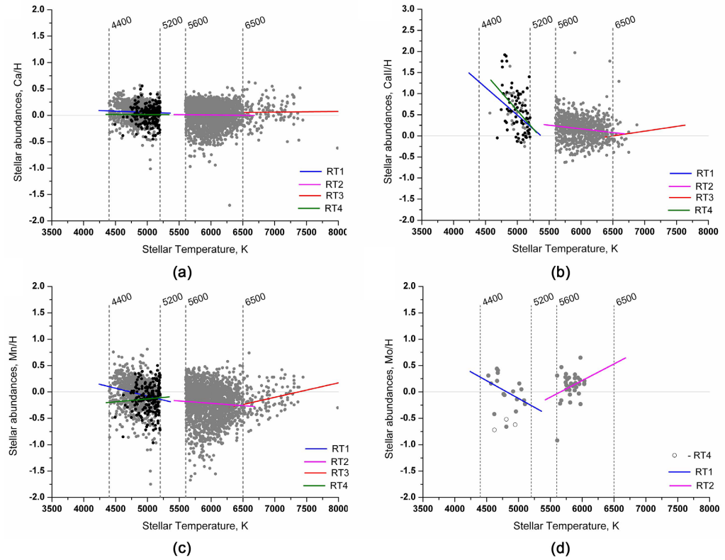
Figure 11. The linear regressions for neutral (ground) and ionized states for Ca (a, b), and for Mn (c), and Mo (d) for RT1-RT4 stellar groups are presented.
