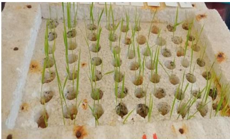
Plate 3. Scoring at 10 th day after salinization
