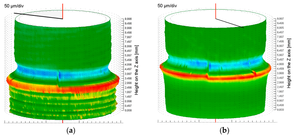
Figure 14. Ball burnished surfaces—the three-dimensional image of the burnishing zone: (a) ( R = 5 \text{ mm} , F = 2.75 \text{ kN} , f_{\text{turn}} = 0.410 \text{ mm/rev} , f_{\text{burn}} = 0.102 \text{ mm/rev} ), (b) ( R = 5 \text{ mm} , F = 2.75 \text{ kN} , f_{\text{turn}} = 0.102 \text{ mm/rev} , f_{\text{burn}} = 0.186 \text{ mm/rev} ).
