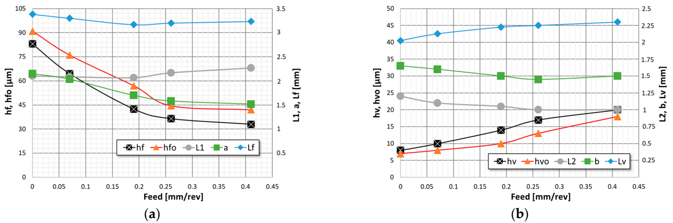
Figure 8. Disc burnishing ( F = 2.75 \text{ kN} , R_k = 5 \text{ mm} )—the impact of the feed on some parameters of the deformation centre determined in: (a) axial section ( h_f , h_{fo} , L_1 , a , L_f ), (b) circumferential section ( h_v , h_{vo} , L_2 , b , L_v ).
