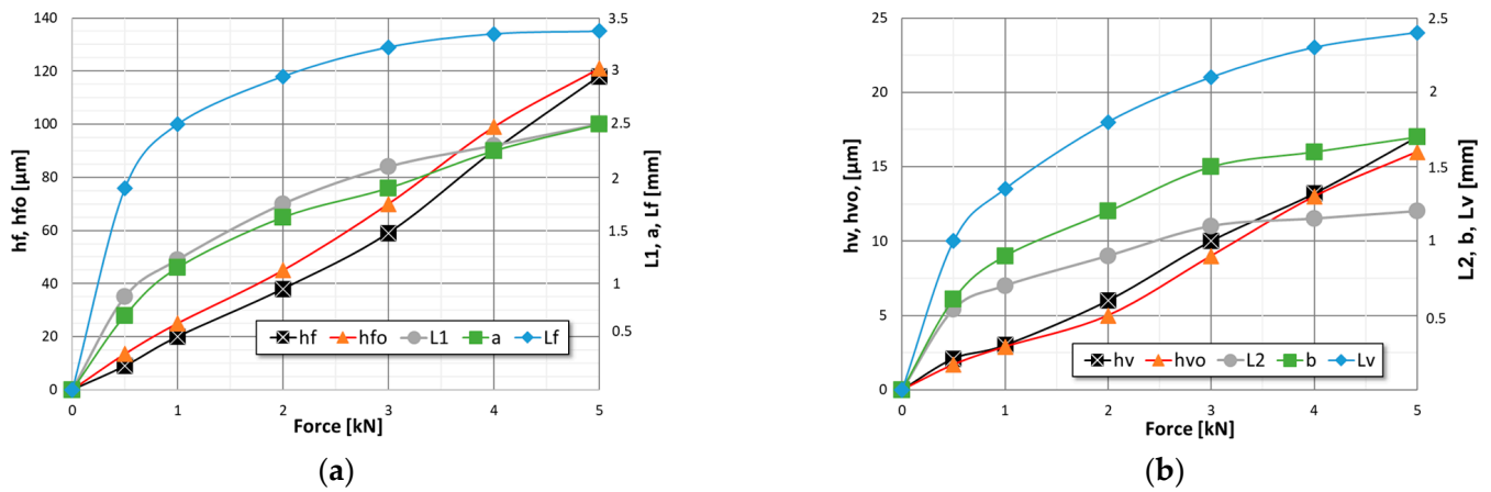
Figure 7. Disc burnishing—the impact of the force on some parameters of the deformation centre ( R_k = 5 \text{ mm} , f_{burn} = 0.102 \text{ mm/rev} ) determined in (a) axial section ( h_f , h_{fo} , L_1 , a , L_f ), (b) circumferential section ( h_v , h_{vo} , L_2 , b , L_v ).
