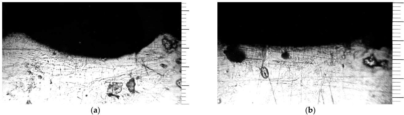
Figure 1. Surface profile: (a) before burnishing—turned zone ( r = 0.4 mm, f_{\text{turn}} = 0.410 mm/rev), (b) ball burnished zone ( R = 5 mm, F = 5 kN, f_{\text{burn}} = 0.410 mm/rev) (magn. 100\times ).
