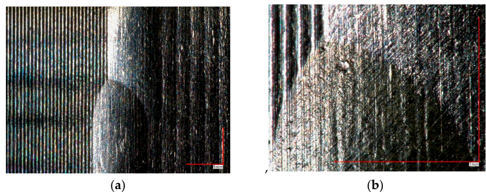
Figure 20. Disc burnishing zone ( R_k = 5 mm, F = 2.75 kN, f_{\text{burn}} = 0.41 mm/rev), mag.: (a) 50 \times ; (b) 200 \times .
