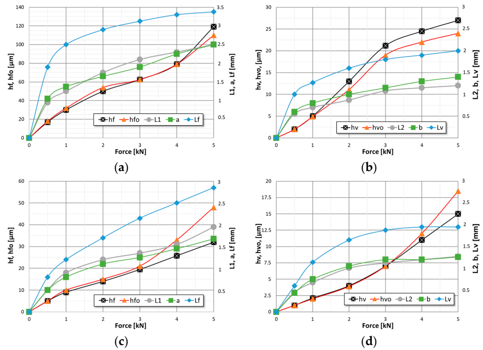
Figure 4. Ball burnishing—the impact of force on some parameters of the deformation centre ( f_{burn} = 0.102 \text{ mm/rev} ) determined in (a,c) axial cross-section ( h_f, h_{fo}, L_1, a, L_f ), (b,d) cross-section peripheral ( h_v, h_{vo}, L_2, b, L_v ), (a,b) ball radius R = 5 \text{ mm} , (c,d) ball radius R = 13.5 \text{ mm} .
