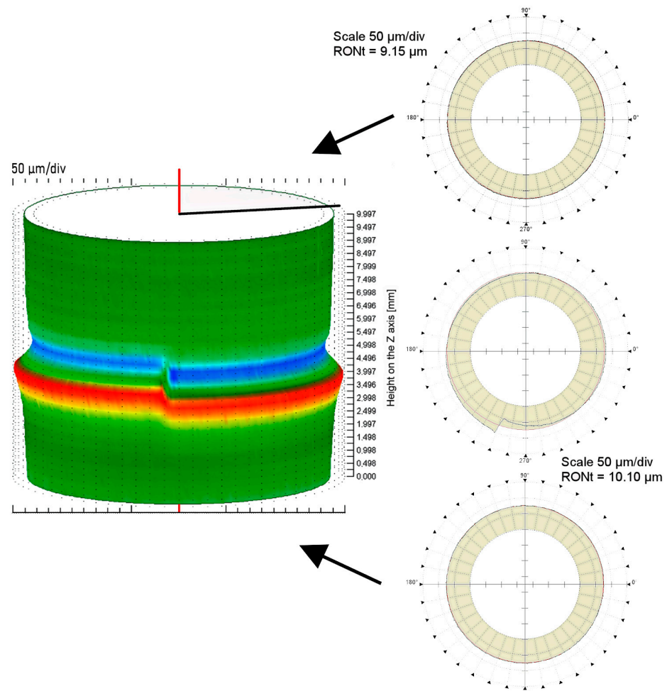
Figure 13. Ball-burnished surface ( R = 5 \text{ mm} , F = 2.5 \text{ kN} , f_{\text{burn}} = 0.5 \text{ mm/rev} )—the three-dimensional image of the burnishing zone.
