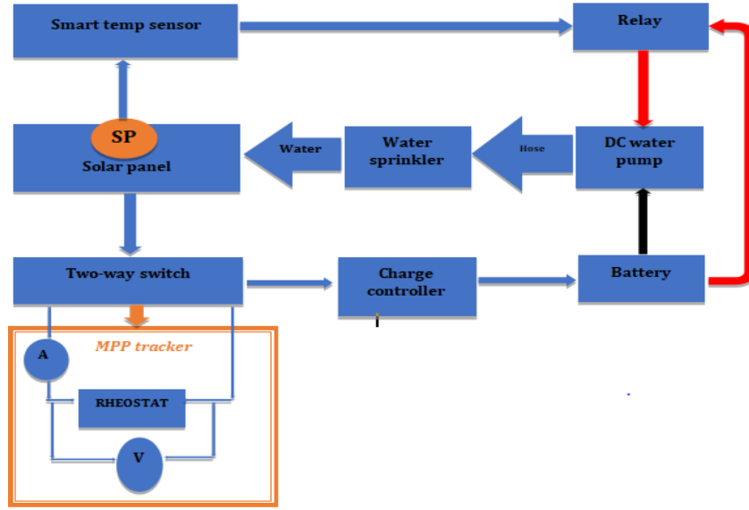
Fig. 1. The experimental setup for the panel installed with automatic cooling mechanism
