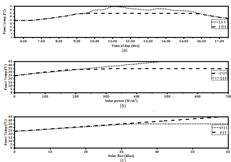
Fig. 3. panel temperature at different time of day with increasing level of solar power and solar flux
