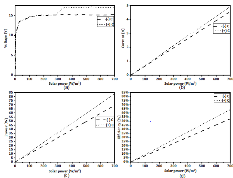
Fig. 4. Influence of cooling mechanism on modules output electrical parameters with respect to solar power
