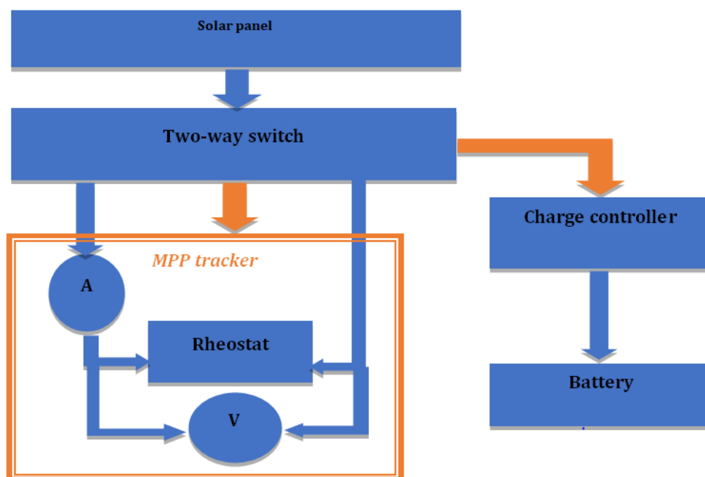
Fig. 2. The experimental setup for solar panel without temperature control
