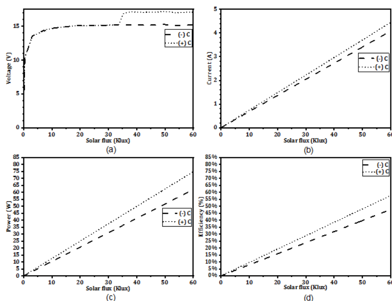
Fig. 5. Influence of cooling mechanism on modules output electrical parameters with respect to solar flux
