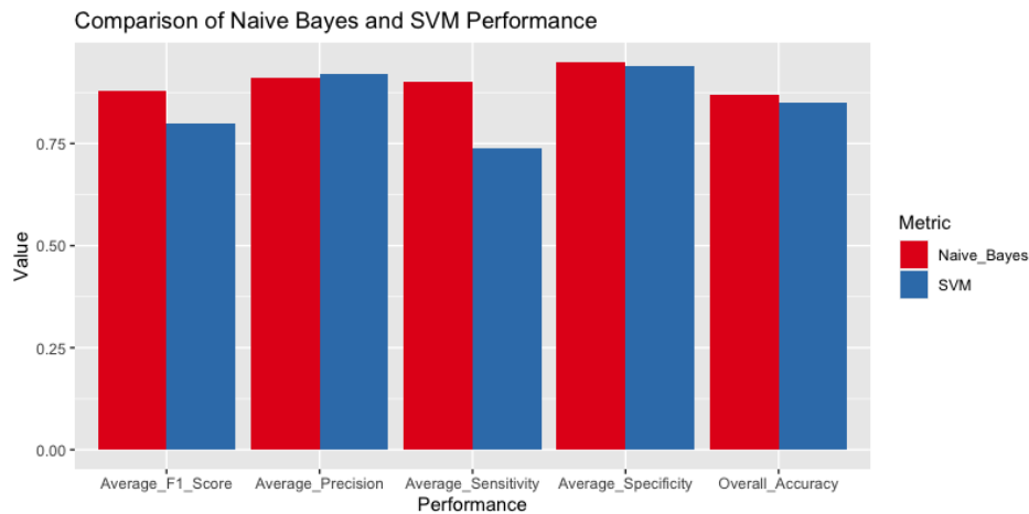
Fig. 5. Metrics for comparison of Naive Bayes and SVM
