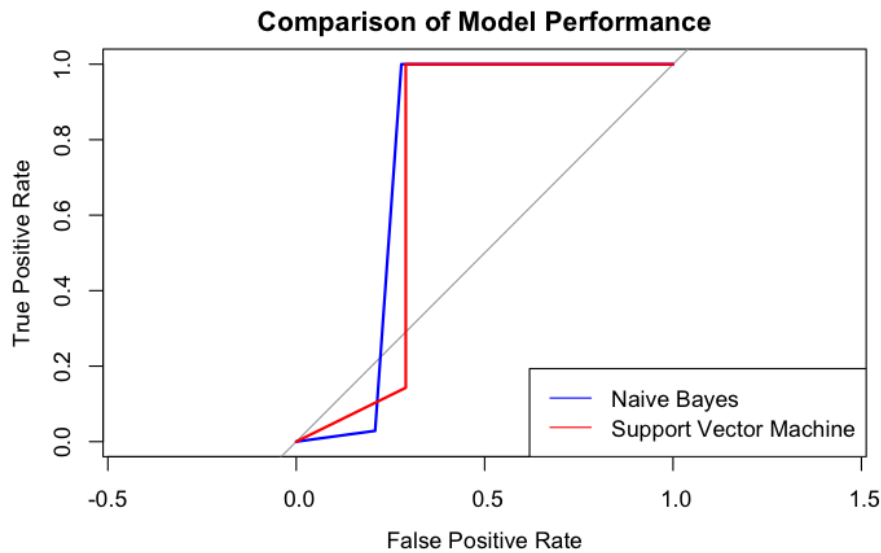
Fig. 4. ROC Curve for Comparison of model performance
