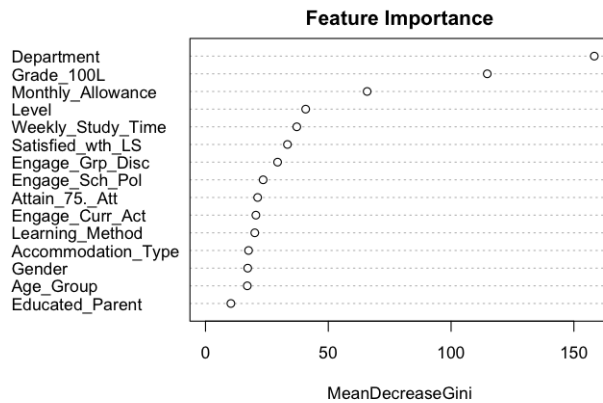
Fig. 6. Important features in model classification
