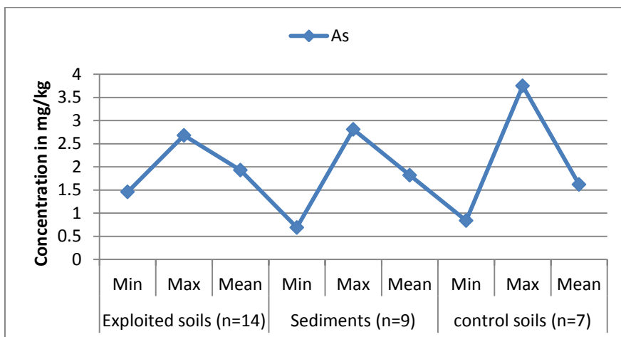
Fig. 5. Variation in concentration of As
