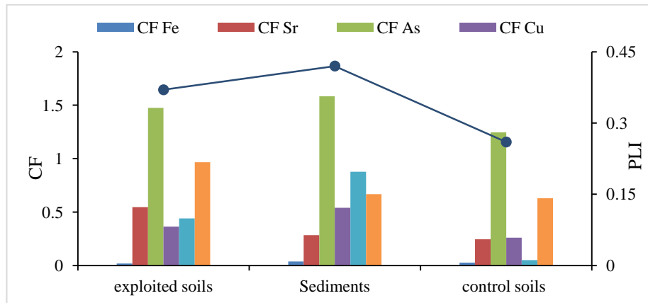
Fig. 8. Variations of the contamination factor (CF) and Pollution load index (PLI)
