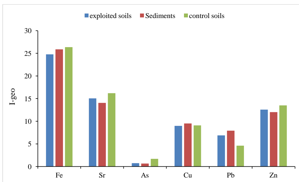
Fig. 7. Variations of the Geo-accumulation Index (I-geo)
