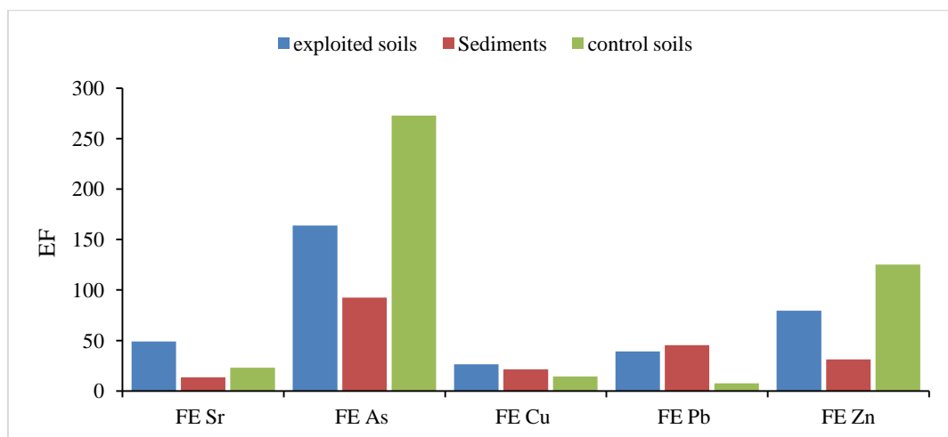
Fig. 6. Variations of the Enrichment Factor (EF)
