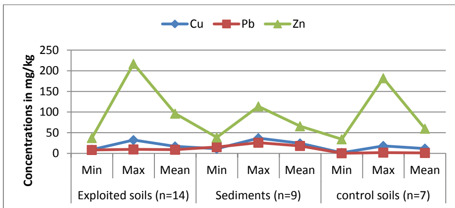
Fig. 4. Variation in concentrations of Cu, Pb and Zn
