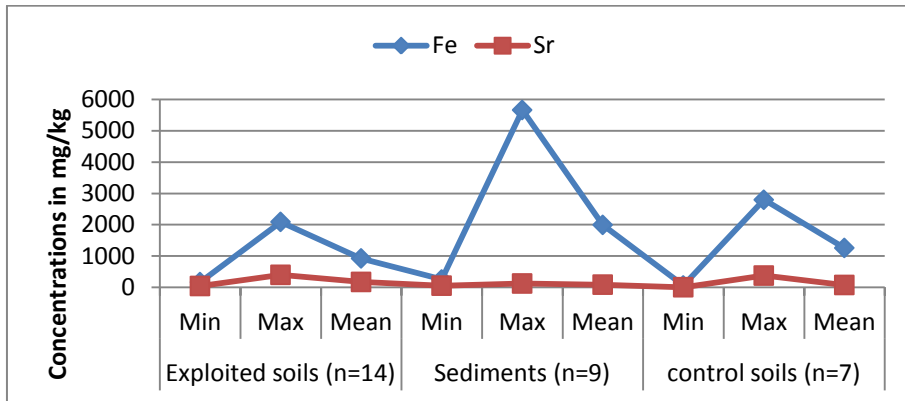
Fig. 3. Variation in concentrations of Fe and Sr
