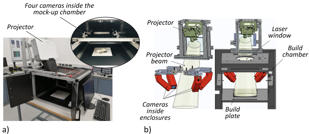
Figure 5. Examples of in-process fringe projection setups: (a) mock-up of a four cameras-one projector system, designed to be integrated in a powder bed fusion (PBF) chamber for the measurement of surface topography (Reproduced from [129], CC BY 4.0.); and (b) CAD design of a multi-sensor measurement system for in-situ defect identification in metal additive manufacturing (Reproduced with permission from [130]. © EUSPEN.), which includes a multi-view fringe projection configuration and a high-speed thermal camera.
