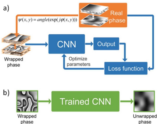
Figure 7. Training and testing the learned phase unwrapping: (a) the unwrapped phase is wrapped to produce training features with which to train and optimise the CNN; (b) the deployed CNN predicts the unwrapped phase on unseen samples (Reproduced with permission from [141]. © The Optical Society).
