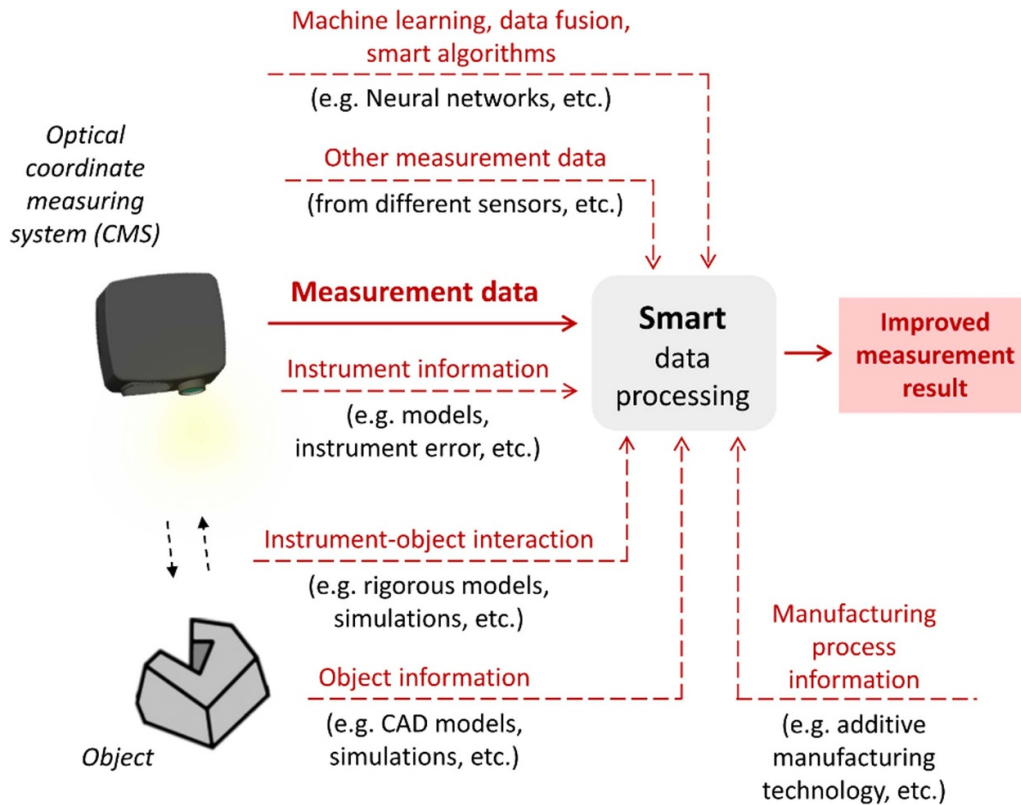
Figure 1. The information-rich metrology (IRM) paradigm (term introduced in [13]). The raw measured data (i.e. the direct result from the measuring instrument) and the final result (i.e. improved optimised measurement result) are indicated with solid red arrows and they are the primary input and the final output of the process; the additional a priori information (for example knowledge of an object/surface being measured, knowledge of the measuring instruments employed and knowledge of the physical interactions/principles underlying the measurement technology itself, with respect to the object being measured, etc) are indicated with dashed red arrows.
