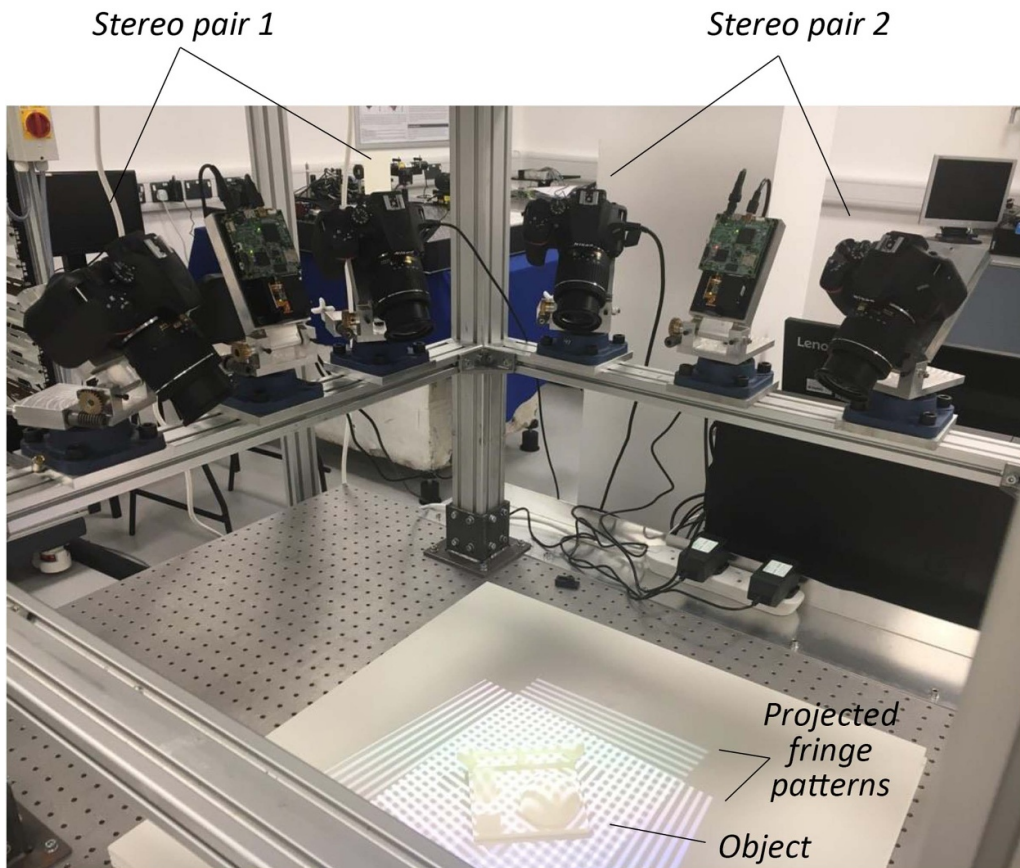
Figure 3. Multi-view systems: fringe projection setup comprised of four DSLR cameras and two projectors for post-processing applications. Reproduced from [115]. © The Author(s). Published by IOP Publishing Ltd. CC BY 4.0.
