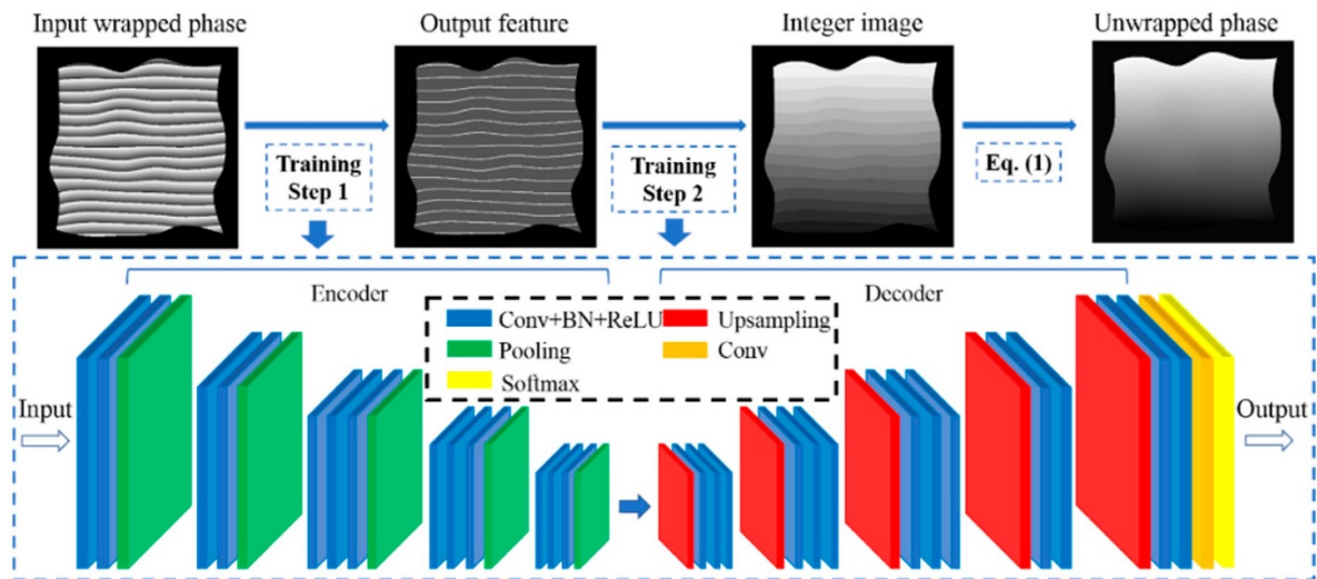
Figure 6. The workflow of the method proposed by Liang et al [140] showing the network architecture for phase unwrapping (Reproduced from [140]. CC BY 4.0.).
