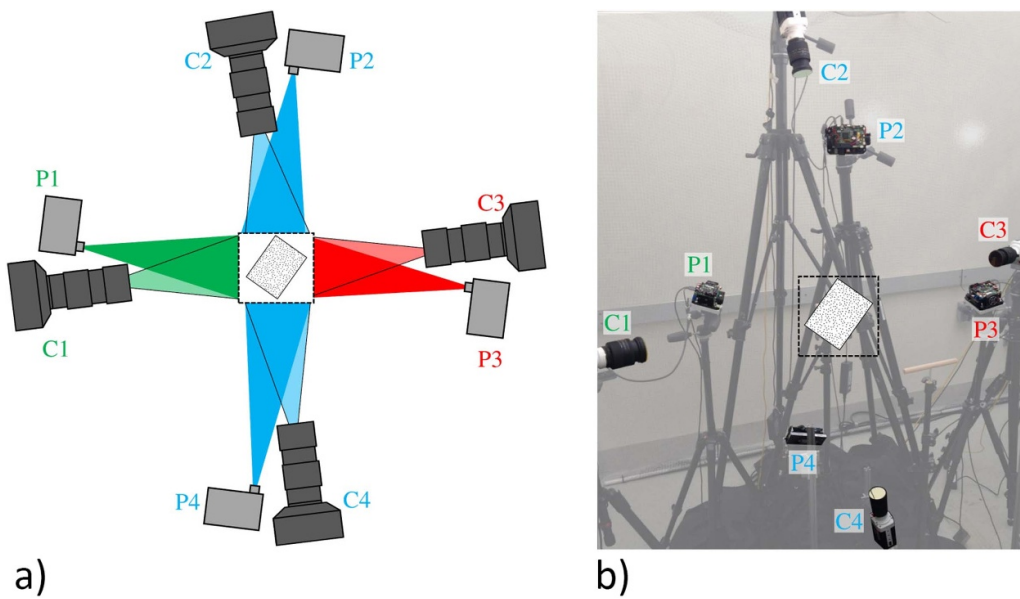
Figure 4. The multi-view structured light system designed by Deetjen and Lentink [125]. (a) Schema showing the configuration of four camera and projector pairs. To reduce cross-talk between the four projected patterns, three different colours matched by camera colour filters for pairs 1–3 were used (green, blue and red respectively). The colour of the 4th pair (blue) is duplicated from the 2nd pair; (b) an image of the actual setup. Reproduced with permission from [125]. © The Optical Society.
