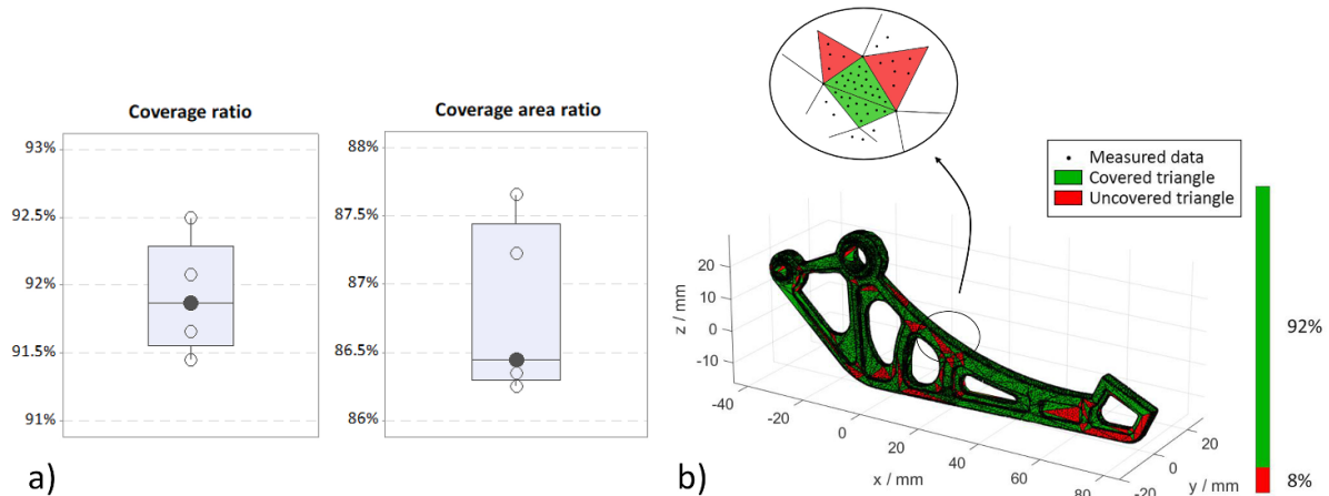
Figure 8. Performance indicators of part coverage from Catalucci et al [86]: (a) boxplots from five measurement repeats indicating coverage ratio, and coverage area ratio respectively (individual results for each of the five repeats, and median); and (b) covered and uncovered triangles rendered using binary colouring projected onto the triangle mesh surface. Reproduced with permission from [86]. © EUSPEN.
