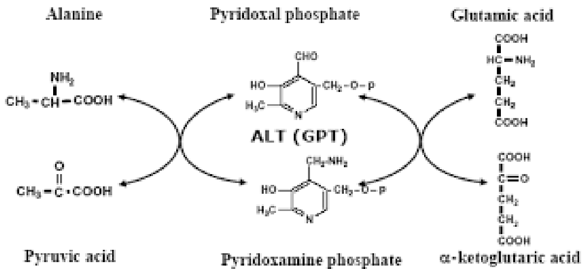
Fig. 3. Showing of the Mechanism of alanine amino transaminase reaction (Tietz et al., 1987, Matinez-Carrion and Peterson, 1970, Karmen et al., 1970)
