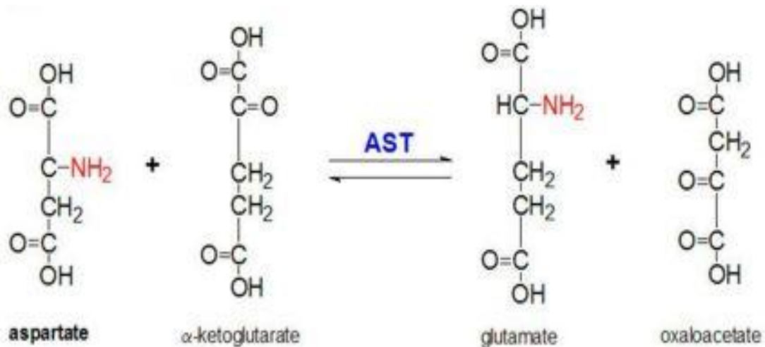
Fig. 2. Showing the Mechanism of aspartate amino transaminase reaction (Tietz et al., 1987, Matinez-Carrion and Peterson, 1970, Karmen et al., 1970)
