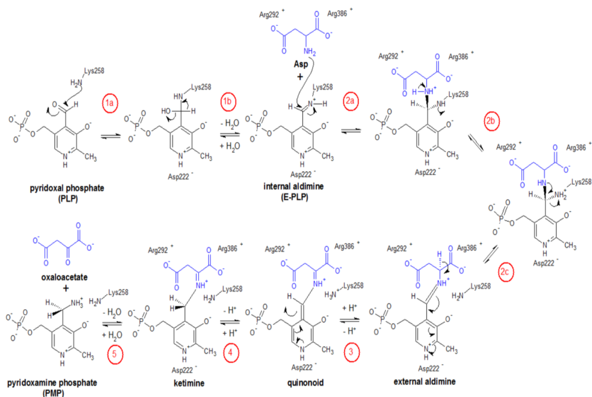
Fig. 4. Showing the steps and stages in mechanism of transamination reaction
