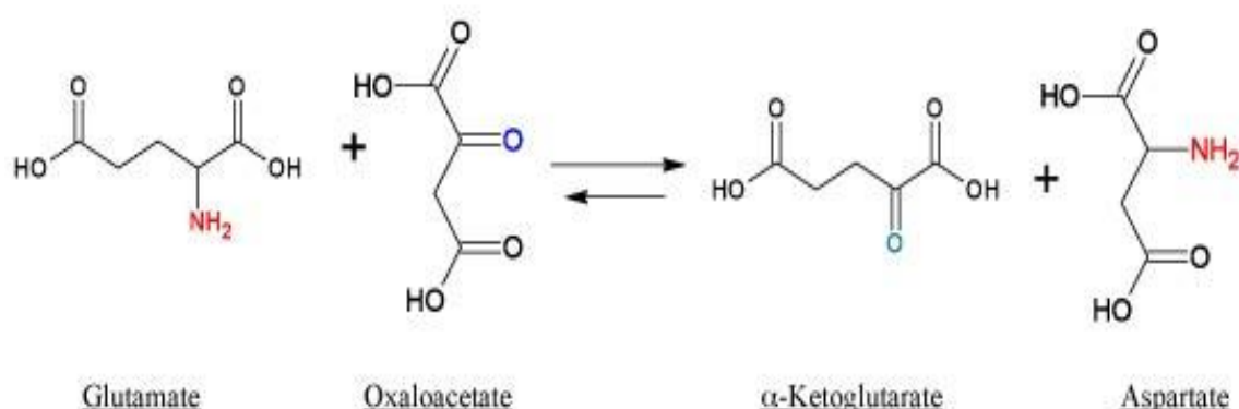
Fig. 1. Showing the principle and Mechanism of transaminase reaction (Tietz et al., 1987, Matinez-Carrion and Peterson, 1970, Karmen et al., 1970)
