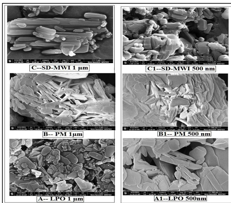
Fig. 8. SEM analysis of LPO (A, A1), PM (B, B1), SD-MWI (C, C1)
