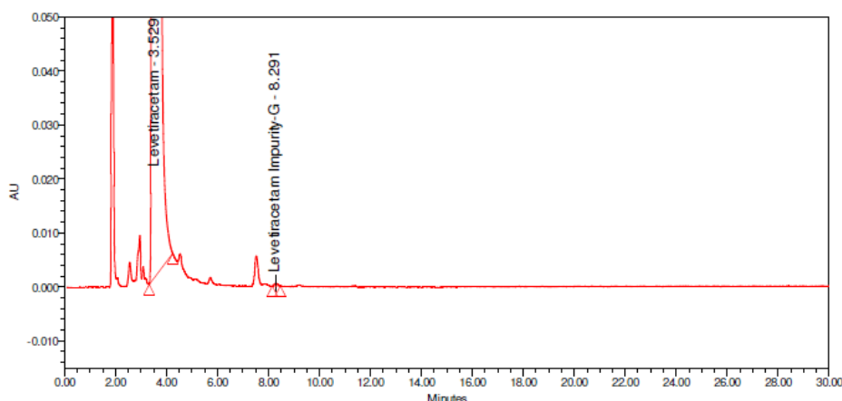
Fig. 6. Typical chromatogram of as such sample
