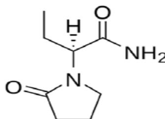
Fig. 1. Chemical structure of Levetiracetam
