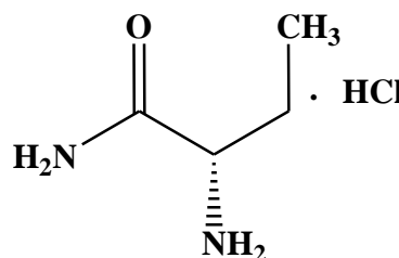
Fig. 2. Chemical structure of impurity-G
