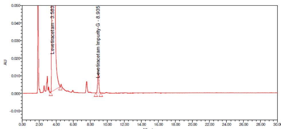
Fig. 7. Impurity-G spiked chromatogram of Levetiracetam
