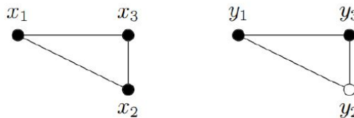
Fig. 2. Hinge domination and total domination on C_3
