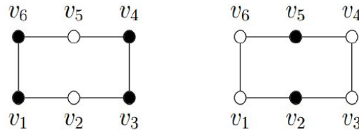
Fig. 1. Total domination and hinge domination on C_6
