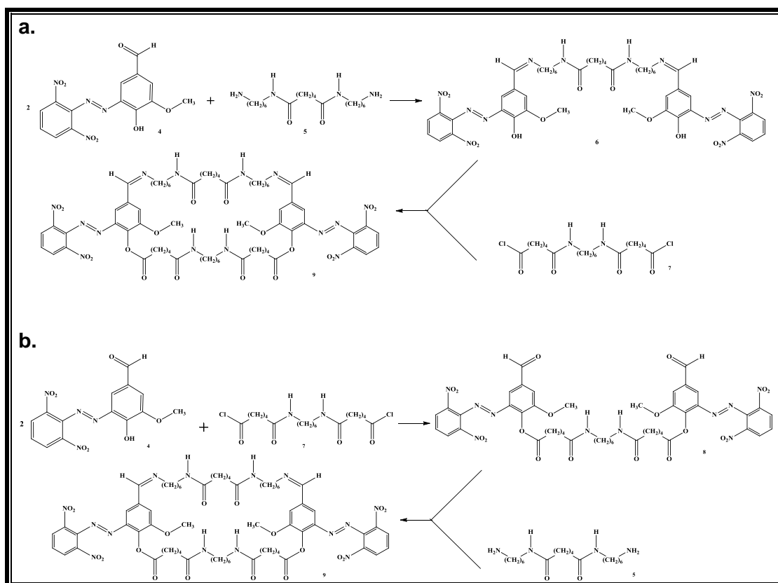
Scheme 3. The pathways for synthesis of 9.
