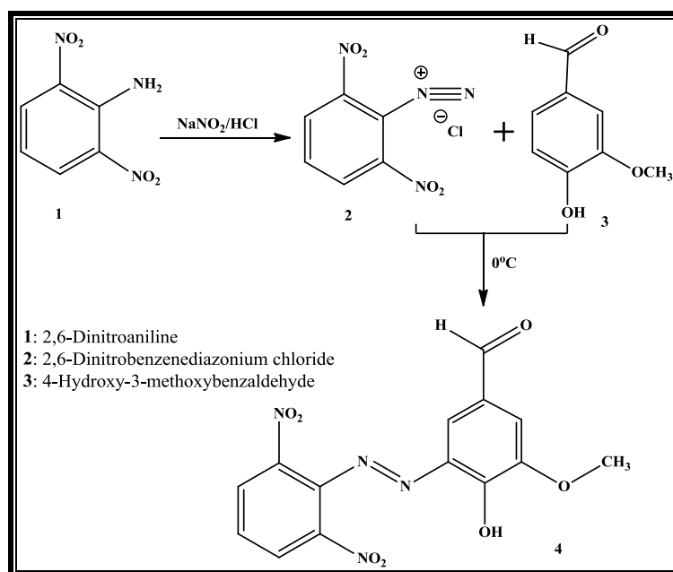
Scheme 2. Synthesis of 4-hydroxy-3-methoxy-5-(2,6-dinitrophenylazo) benzaldehyde 4
