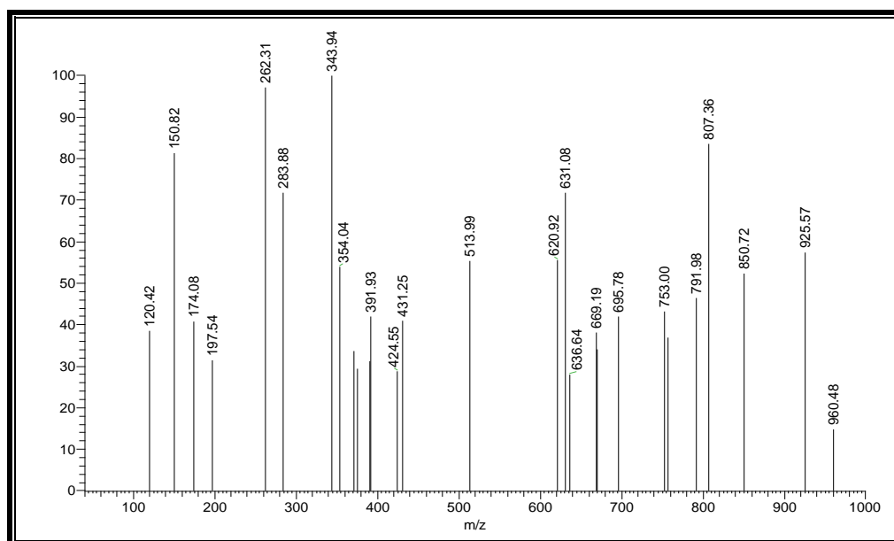
Fig. 3. The Mass Spectrum of new synthesized amide 9
