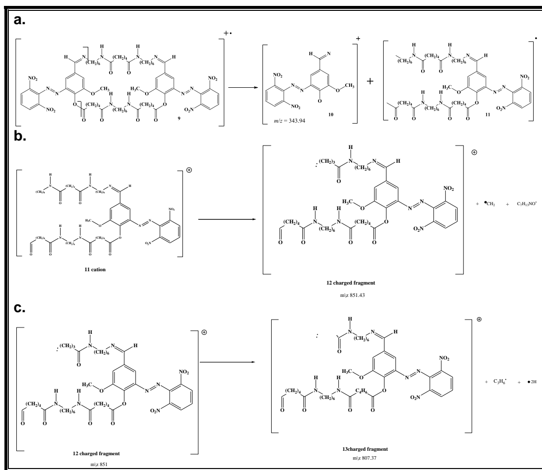
Fig. 4. The fragments a. 10 and 11, b. 12, and c. 13 of compound 9
