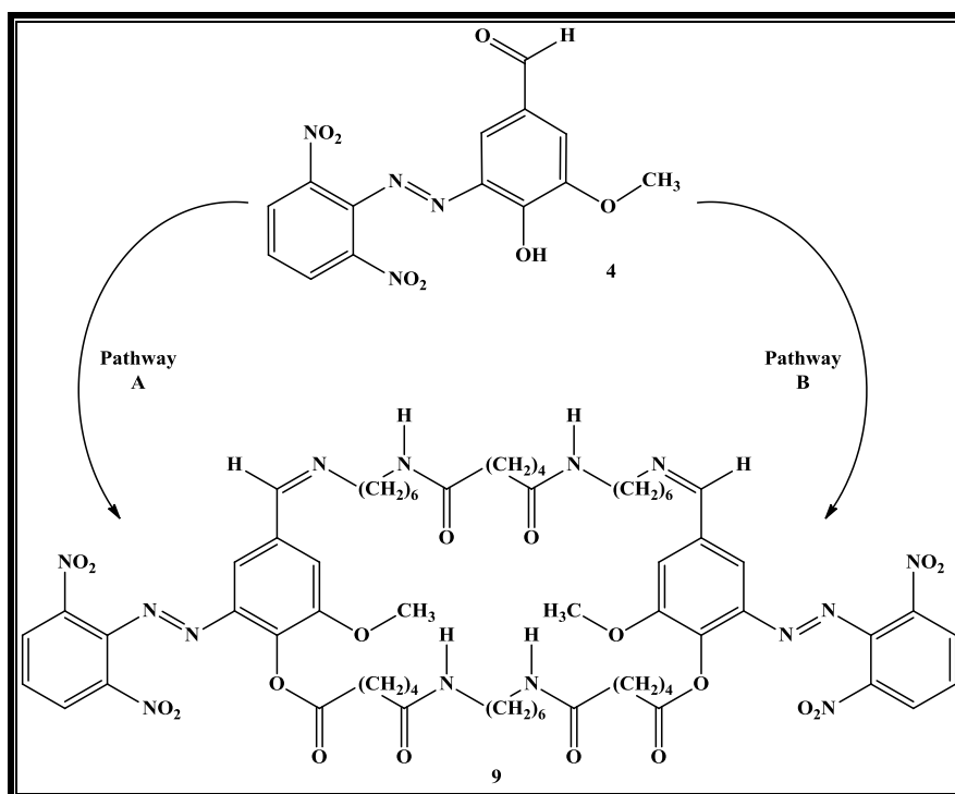
Scheme 1. The new synthesized of amide 9
