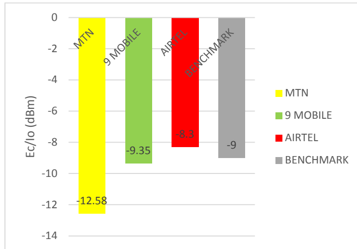
Fig. 1. Mean values of E_c/I_o for the networks under study
