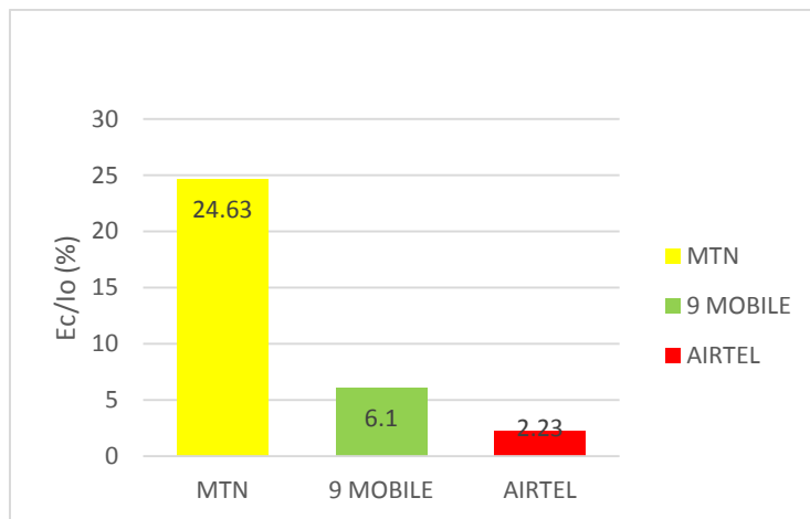
Fig. 8. Percentage of Ec/Io at -40dB to -15dB for the networks under study
