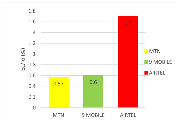
Fig. 3. Percentage of E_c/I_o at -3dB to 0dB for the networks under study
