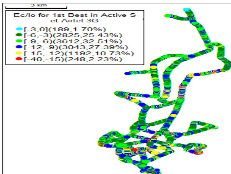
Fig. 9. Received signal quality plots of Ec/Io for Airtel network
