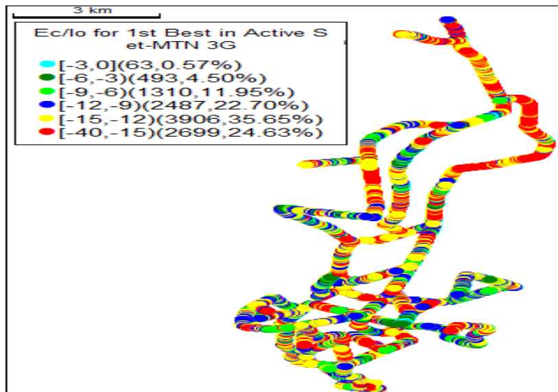
Fig. 10. Received signal quality plots of Ec/Io for MTN network
