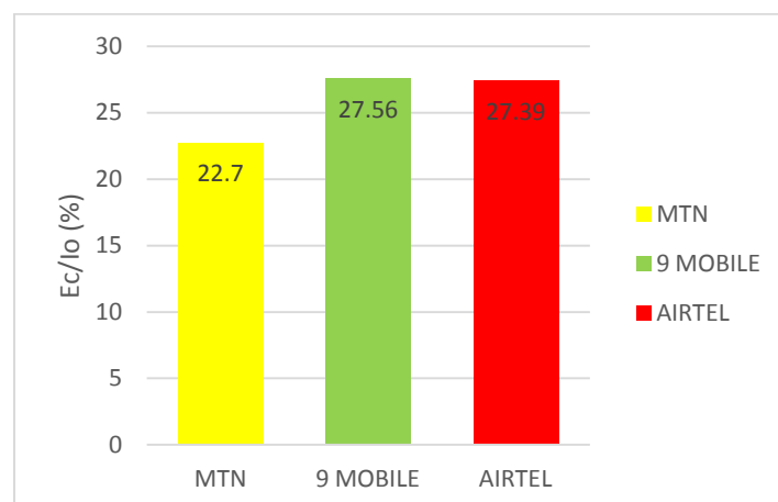
Fig. 6. Percentage of Ec/Io at -12dB to -9dB for the networks under study
