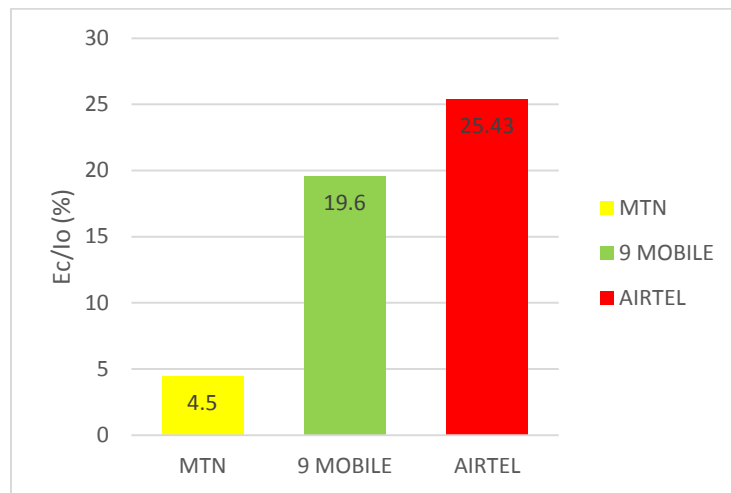
Fig. 4. Percentage of Ec/Io at -6dB to -3dB for the networks under study
