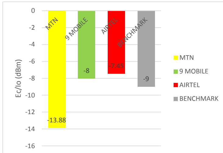
Fig. 2. Most occurring values of E_c/I_o for the networks under study
