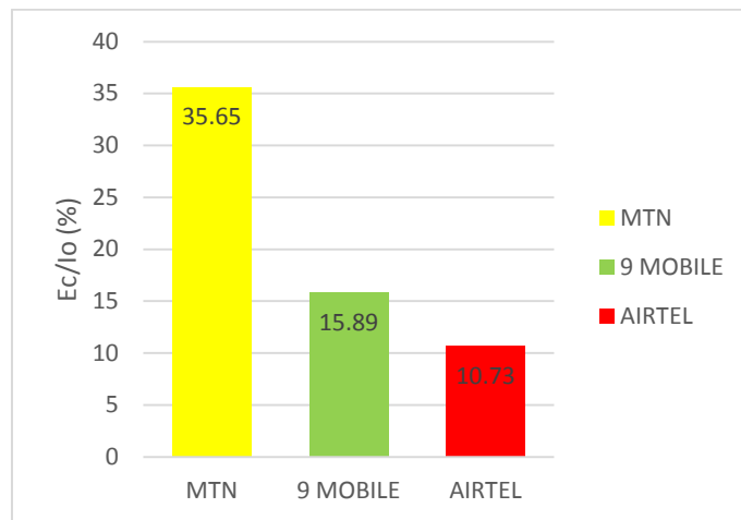
Fig. 7. Percentage of Ec/Io at -15dB to -12dB for the networks under study
