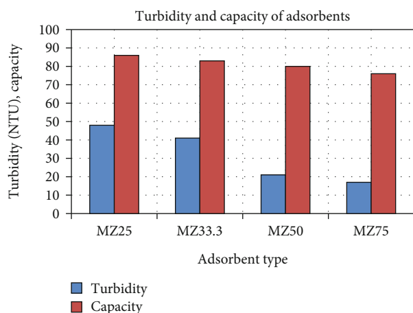
FIGURE 4: Turbidity of filtrate and adsorption capacity of magnetic zeolites.
