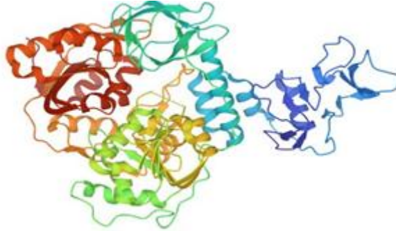
Fig. 1. Helicase Receptor Structure with PDB code 6ZSL
