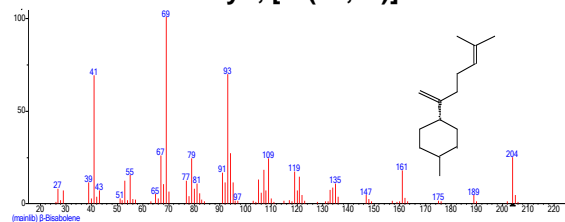
Structure of beta-Bisabolene
