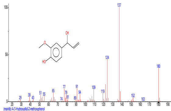
Structure of 4-(1-Hydroxyallyl)-2-methoxyphenol
