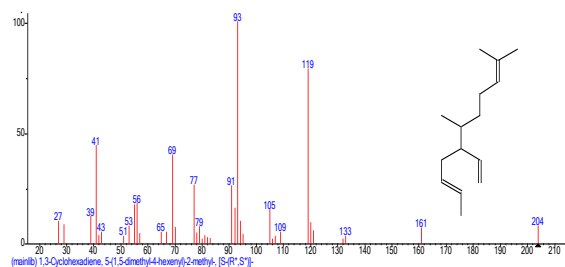
Structure of 1,3-Cyclohexadiene, 5-(1,5-dimethyl-4-hexenyl)-2-methyl-, [S-(R*,S*)]-
