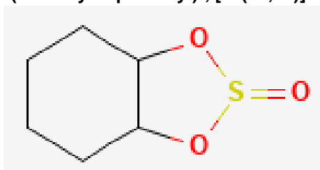
Structure of 1,2-Cyclohexanediol, cyclic sulfite, trans-
