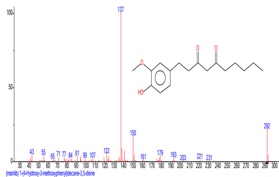
Structure of 1-(4-Hydroxy-3-methoxyphenyl) decane-3,5-dione
