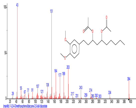
Structure of 1-(3,4-Dimethoxyphenyl)decane-3,5-diy diacetate
