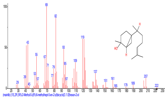
Structure of (1S,2R,5R)-2-Methyl-5-((R)-6-methylhept-5-en-2-yl)bicyclo[3.1.0]hexan-2-ol
