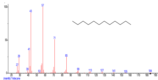
Structure of Tridecane
