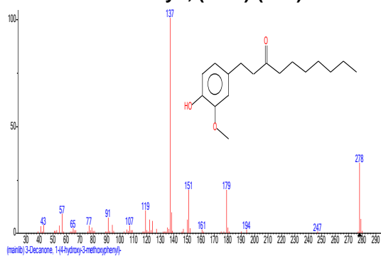
Structure of 3-Decanone, 1-(4-hydroxy-3-methoxyphenyl)-
