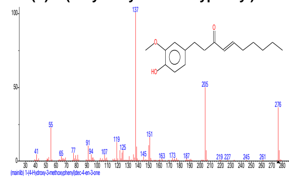
Structure of 1-(4-Hydroxy-3-methoxyphenyl) dec-4-en-3-one
