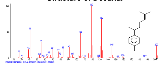
Structure of Benzene, 1-(1,5-dimethyl-4-hexenyl)-4-methyl-
