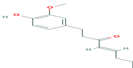
Structure of 1-(4-Hydroxy-3-methoxyphenyl) oct-4-en-3-one
