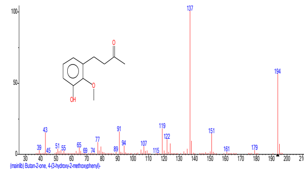
Structure of Butan-2-one, 4-(3-hydroxy-2-methoxyphenyl)-
