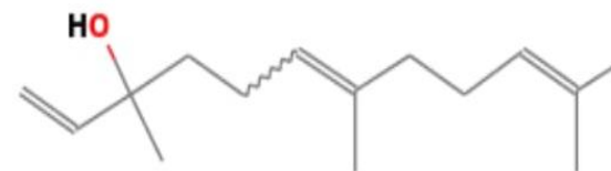
Structure of Cyclohexene, 3-(1,5-dimethyl-4-hexenyl)-6-methylene-, [S-(R*,S*)]-
