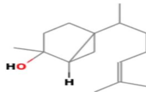
Structure of trans-Sesquisabinene hydrate
