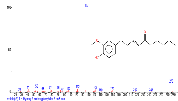
Structure of (E)-1-(4-Hydroxy-3-methoxyphenyl) dec-3-en-5-one
