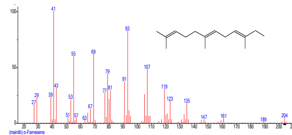
Structure of alpha-Farnesene
