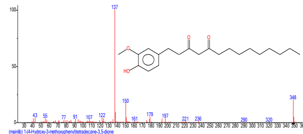
Structure of 1-(4-Hydroxy-3-methoxyphenyl) tetradecane-3,5-dione
