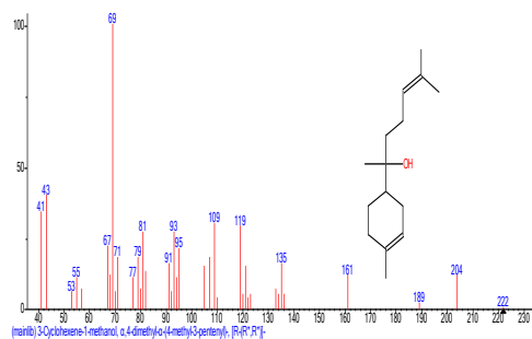
Structure of 3-Cyclohexene-1-methanol, .alpha., 4-dimethyl-.alpha.-(4-methyl-3-pentenyl)-, [R-(R*,R*)]-
