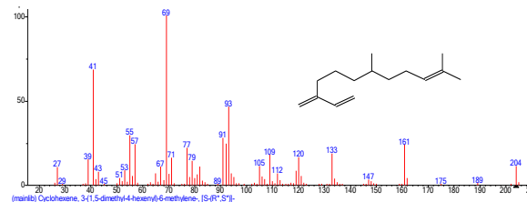
Structure of Cyclohexene, 3-(1,5-dimethyl-4-hexenyl)-6-methylene-, [S-(R*,S*)]-
