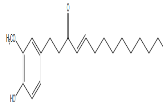
Structure of (E)-1-(4-Hydroxy-3-methoxyphenyl) tetradec-4-en-3-one
