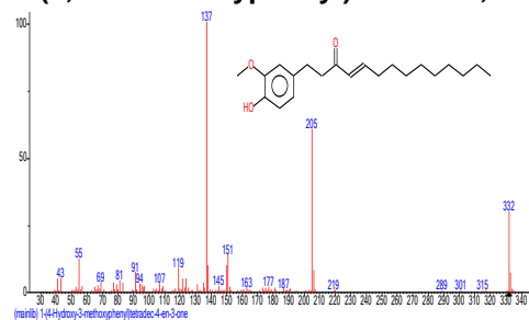
Structure of 1-(4-Hydroxy-3-methoxyphenyl) tetradec-4-en-3-one
