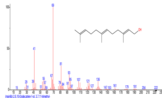
Structure of 2,6,10-Dodecatrien-1-ol, 3,7,11-trimethyl-
