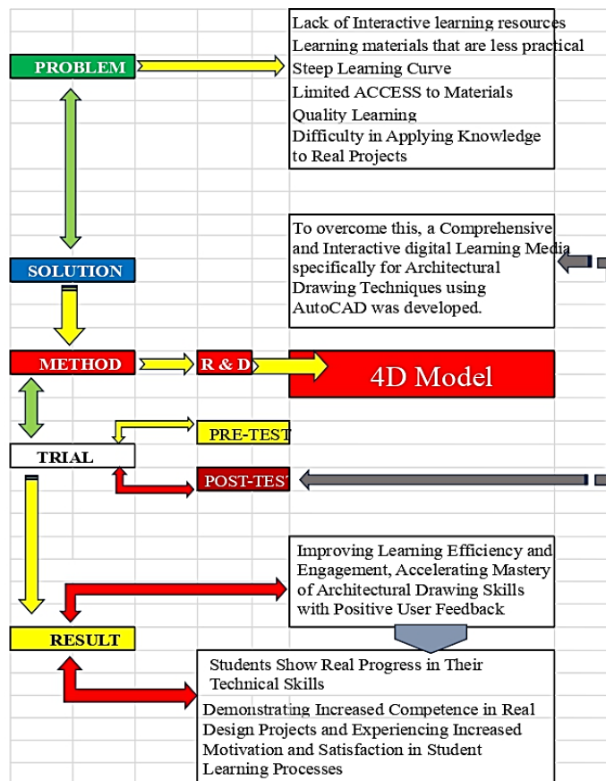
Fig. 2. Thinking framework
