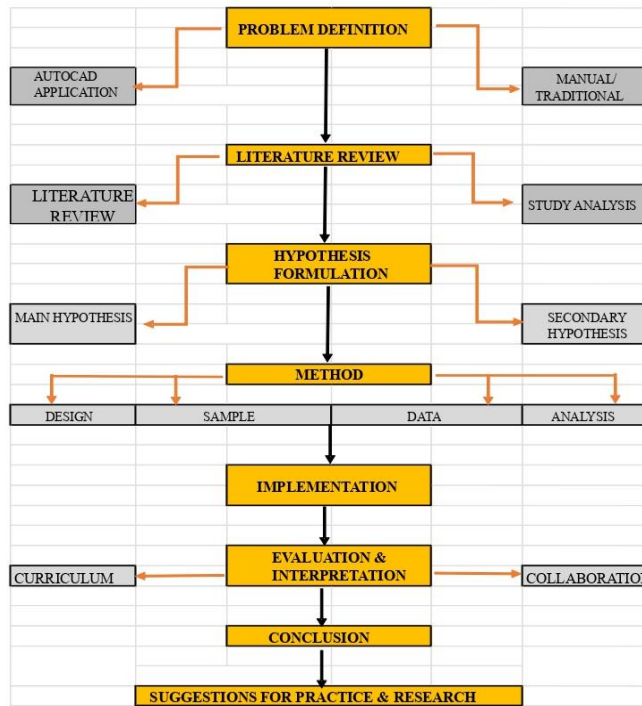
Fig. 1. Hypothesis framework
