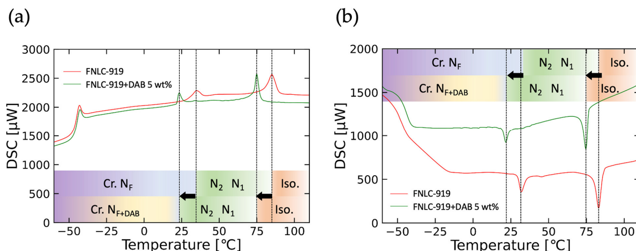
Figure 1. Thermal analysis of phase transition temperatures influenced by the addition of DAB to FNLC-919. A DSC assessment was undertaken to determine how a 5 wt% mixture of FNLC-919 and DAB modulates the phase transition relative to pristine FNLC-919. (a) Exothermic peaks during the temperature decrease. (b) Endothermic peaks during the temperature increase. The respective masses during the measurements were 8.20 mg for the pristine sample and 8.23 mg for the mixture, with a controlled temperature rate of 10 °C/min.
