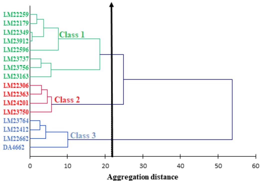
Fig. 2. Hierarchical ascending classification of hybrid progenies based on bunch and palm oil yield components
