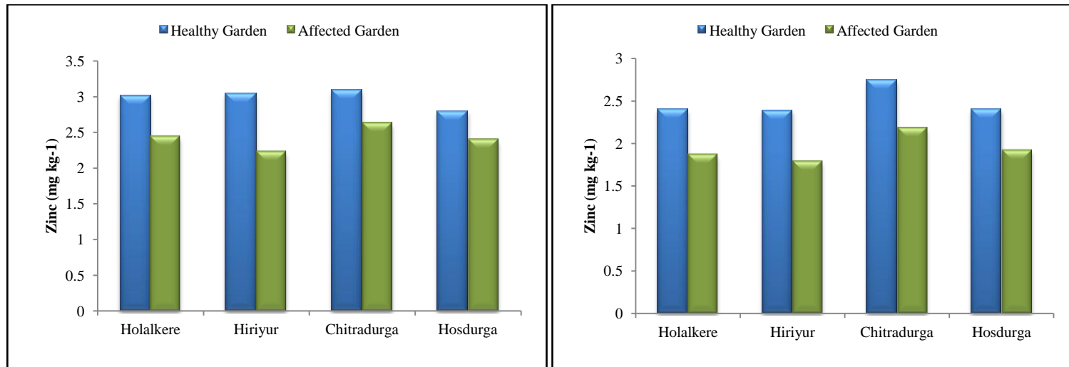
Fig. 3. Average zinc content in soils under healthy and hidimundige affected arecanut gardens of Chitradurga district (a) surface layers (b) subsurface layers
