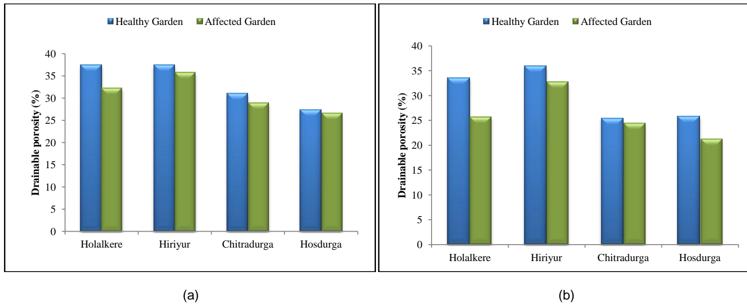
Fig. 2. Drainable porosity in surface layers of soils under healthy and hidimundige affected arecanut gardens of Chitradurga district (a) in surface layers (b) in subsurface layers
