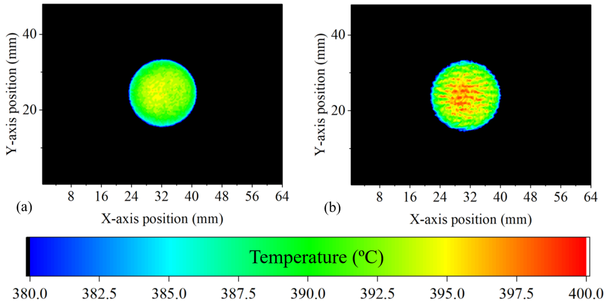
Figure 7. Thermal images of a 20 mm diameter target aperture placed in front of a furnace at a temperature of 395 ^{\circ}\text{C} , using (a) InGaAs APD and (b) InGaAs photodiode-based scanners.
