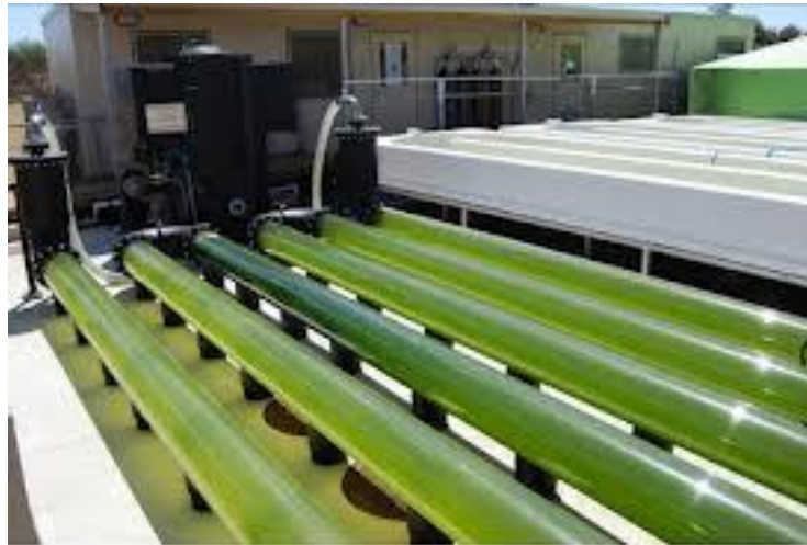
Fig. 7. Tubular photobioreactor [189]
