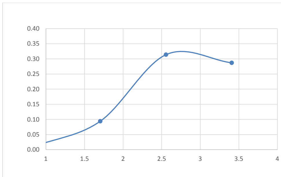
Fig. 5. Tip speed ratio vs coefficient of performance
