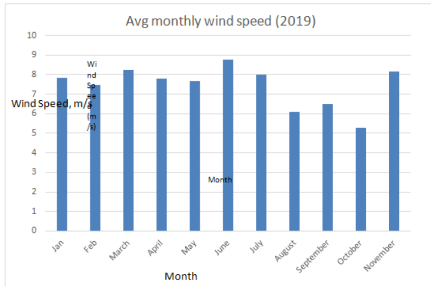
Fig. 2. Monthly Average Offshore Wind Speed in meters/sec
