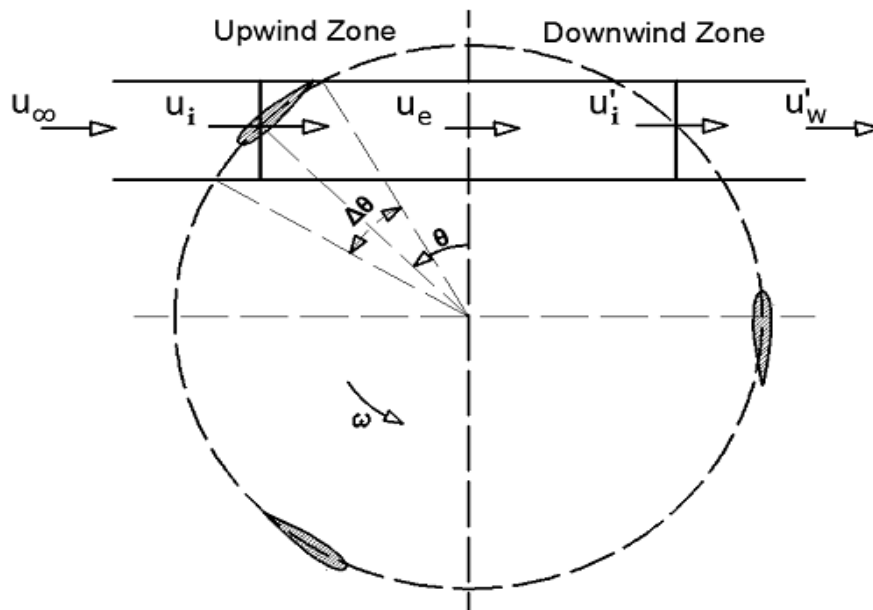
Fig. 4. Double multiple streamtube model
