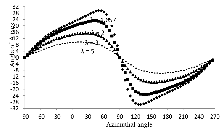
Fig. 3. Changing angle of attack with rotation at different tip speed ratios
