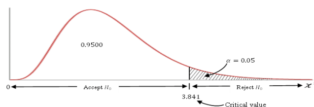
Fig. 2. Critical value at 0.05 significance level
