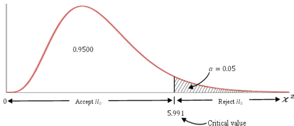
Fig. 5. Critical value at 0.05 significance level
