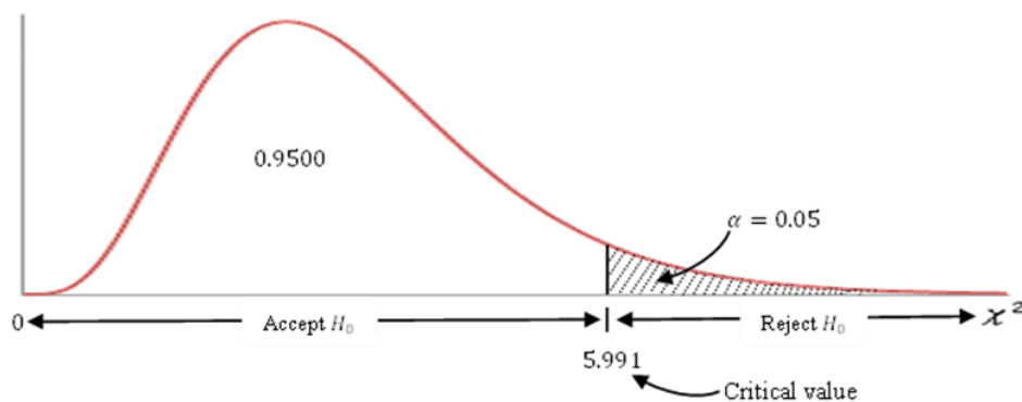
Fig. 4. Critical value at 0.05 significance level
