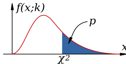
Fig. 1 A graph of a chi-square ( \chi^2 ) distribution
