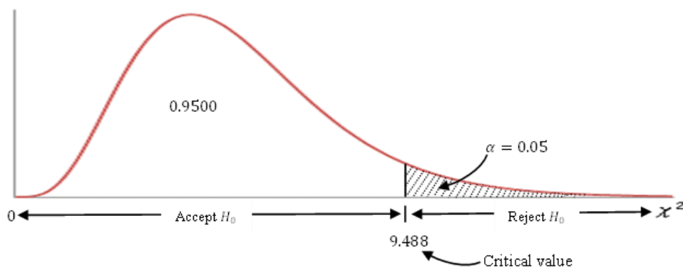
Fig. 3. Critical value at .05 significant level
