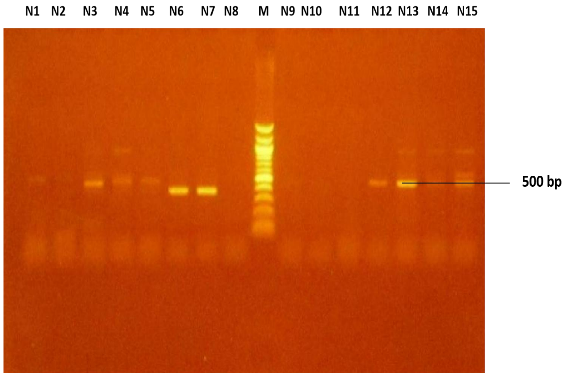
Plate 2. Agarose gel electrophoresis of CTX-M gene amplification by Salmonella isolates from street vended food Lane N1, N3-N7 and N13-N15 represents the positive CTX-M gene bands (500bp). Lane M represents the 1 kb Molecular ladder.
