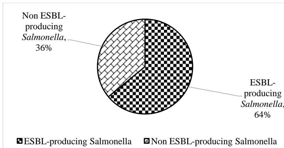
Fig. 3. Occurrence of ESBL- and Non ESBL-Producing Salmonella sp. in food samples
