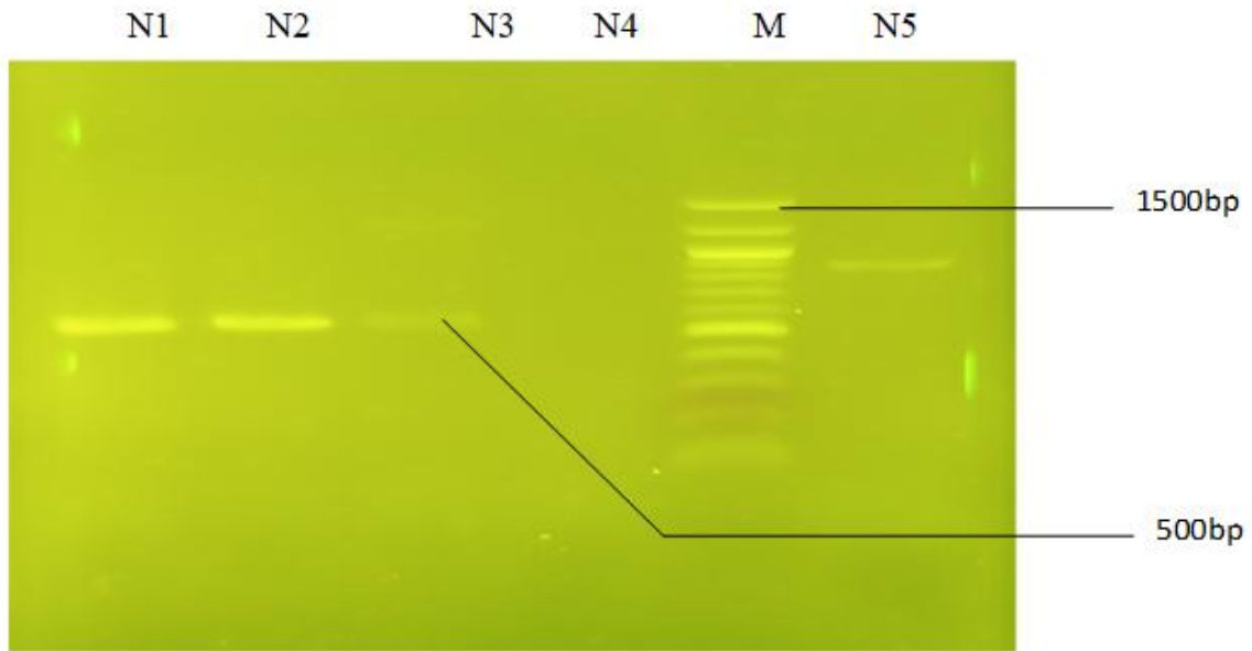
Plate 5. Agarose Gel Electrophoresis of CTX-M gene amplification by Salmonella isolates from street vended food
