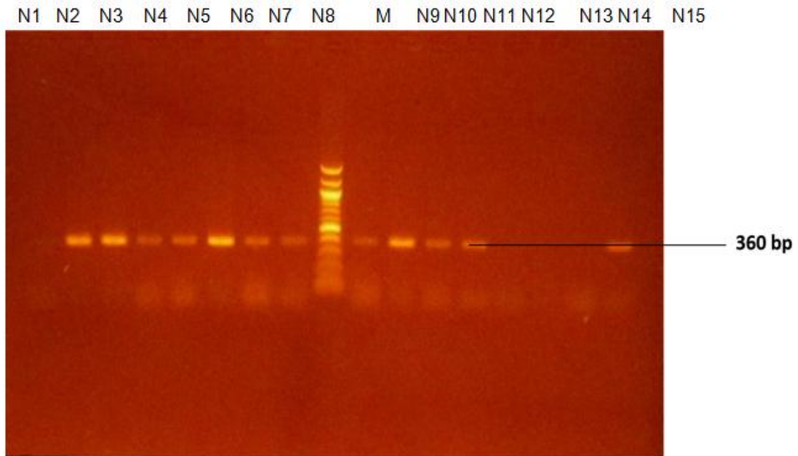
Plate 3. Agarose gel electrophoresis of TEM gene amplification by Salmonella isolates from street vended food
