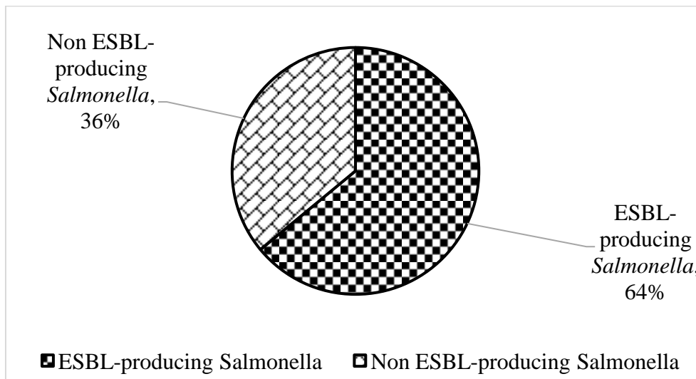
Fig. 2. Occurrence of ESBL- and Non ESBL-Producing Salmonella sp. in food handlers
