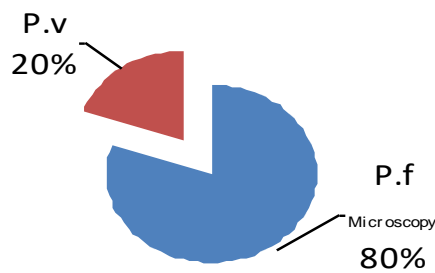
Fig. 7. Malaria types
