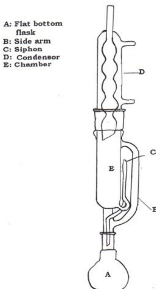
Fig. 3. Soxhlet extractor
